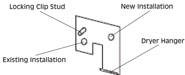
OPTIONAL WALL MOUNTING BRACKET
